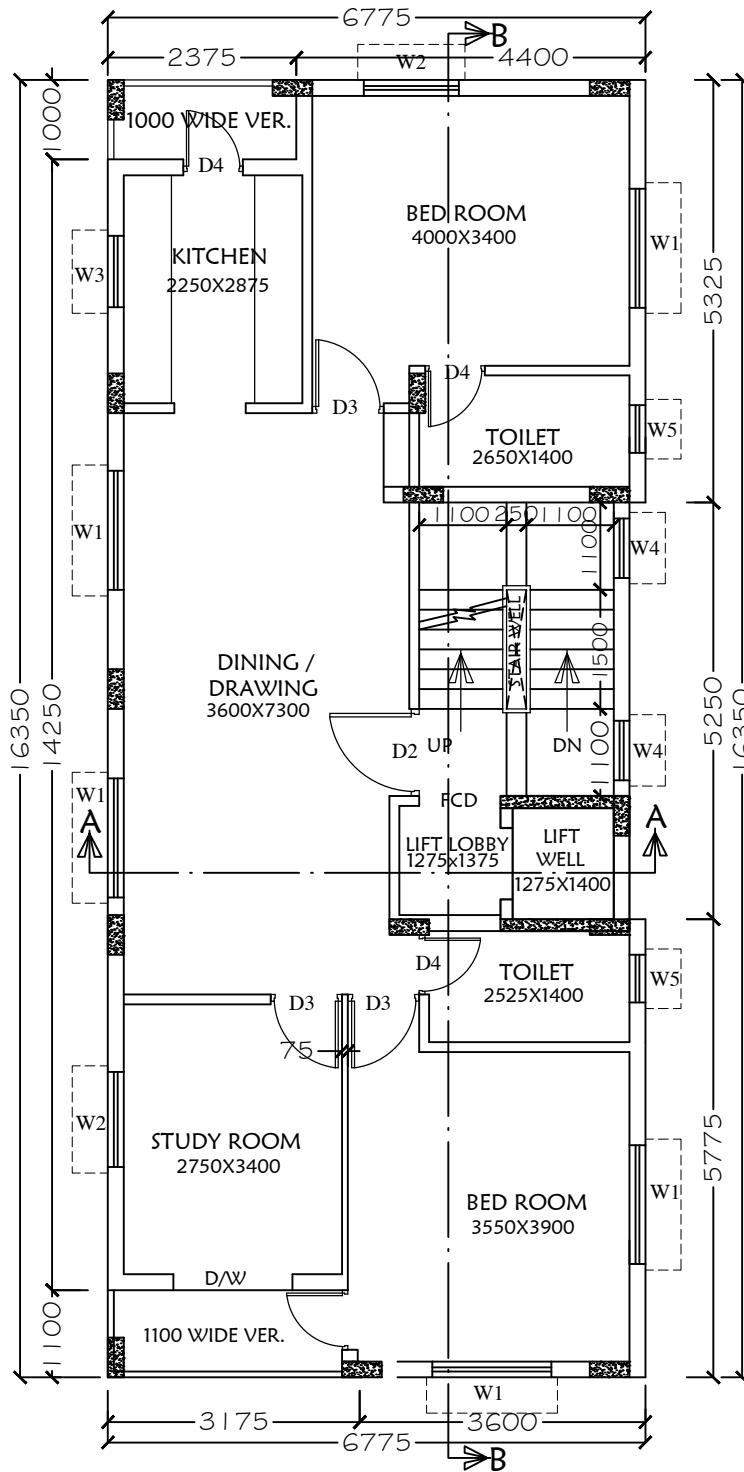
TYPICAL FLOOR PLAN(1ST TO 4TH)
