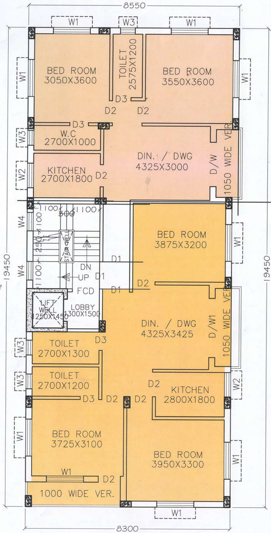
TYPICAL FLOOR PLAN (1st, 2nd, 3rd & 4th Floor)
